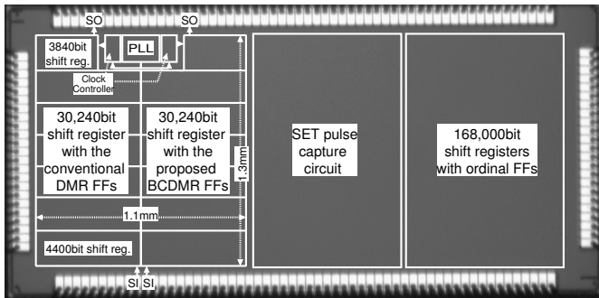
Fig. 6. Chip photo and floorplan.
